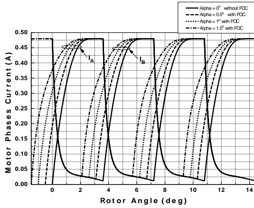
Fig.3 Motor phases current versus rotor angle during four step angles
