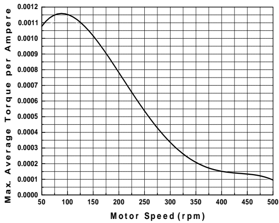
Fig.16 Maximum average torque per ampere versus motor speed (advance turn-on)
