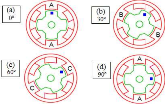
Fig.1 A one quarter revolution of a 2-phase VR step motor
