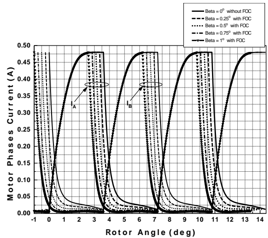
Fig.6 Motor phases current versus rotor angle during four step angles
