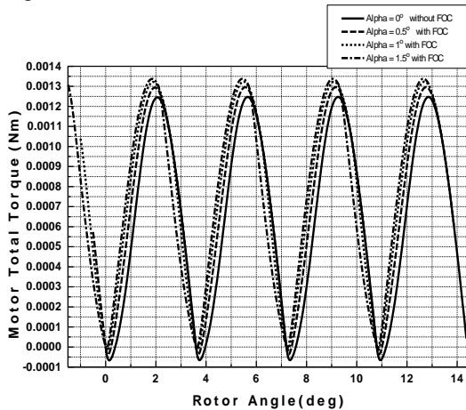
Fig.4 Motor total torque versus rotor angle during four step angles
