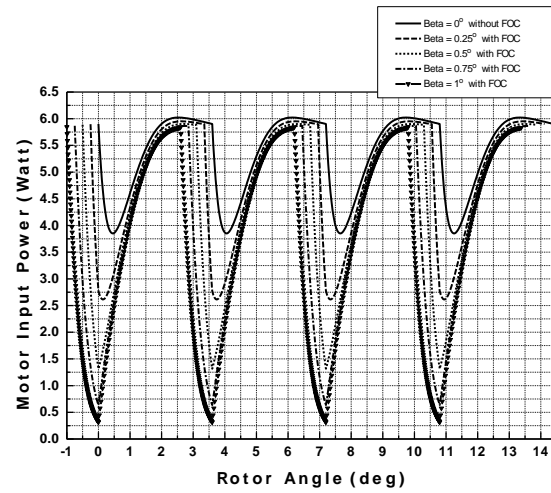
Fig.9 Motor input power versus rotor angle during four step angles
