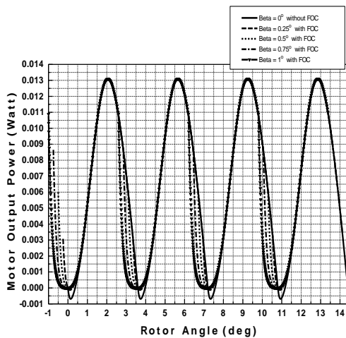
Fig.8 Motor output power versus rotor angle during four step angles
