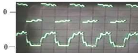
Fig.21 Stator voltage & Stator current Horizontal: Time 20 ms/div & Freq. 43 step/s. Vertical: Upper Trace (Stator voltage) 10 V/div Lower Trace (Stator current) 0.2 A/div
