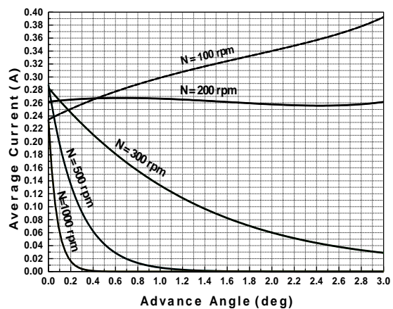
Fig.10 Motor phases average current versus advance turn-on at different speeds
