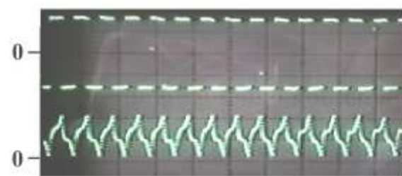
Fig.23 Stator voltage & Stator current Horizontal: Time 20 ms/div & Freq. 145 step/s. Vertical: Upper Trace (Stator voltage) 10 V/div Lower Trace (Stator current) 0.2 A/div
