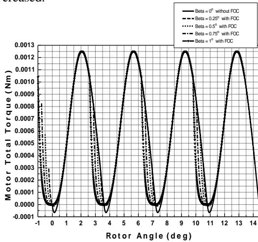
Fig.7 Motor total torque versus rotor angle during four step angles
