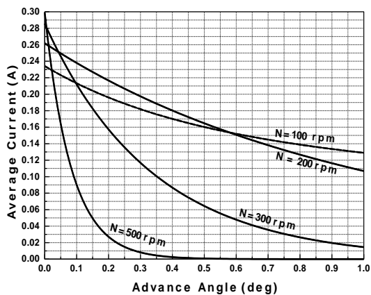
Fig.13 Motor phases average current versus advance turn-off angle at different speeds
