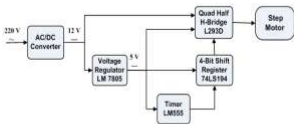
Fig.18 A brief schematic diagram of experimental connections
