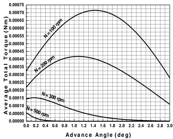
Fig.11 Average total torque versus advance turn-on angle at different speeds
