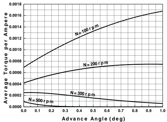
Fig.15 Average torque per ampere versus advance turn-off angle at different speeds
