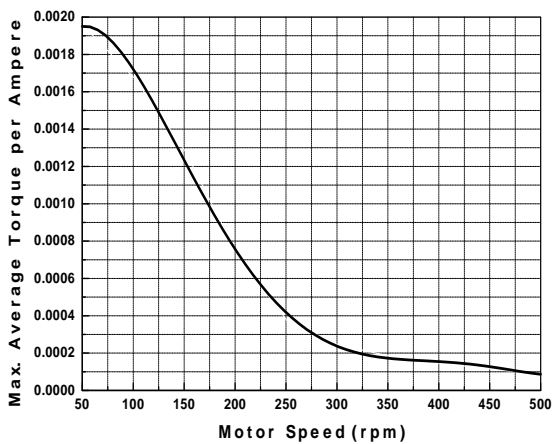
Fig.17 Maximum average torque per ampere versus motor speed (advance turn-off)
