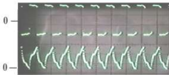
Fig.22 Stator voltage & Stator current Horizontal: Time 20 ms/div & Freq. 100 step/s. Vertical: Upper Trace (Stator voltage) 10 V/div Lower Trace (Stator current) 0.2 A/div
