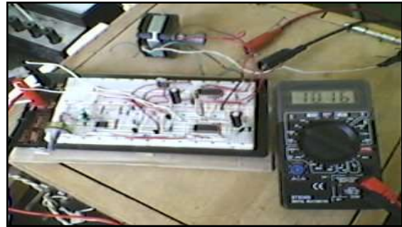
Fig.19 A photograph of the experimental setup of stepper motor driver
