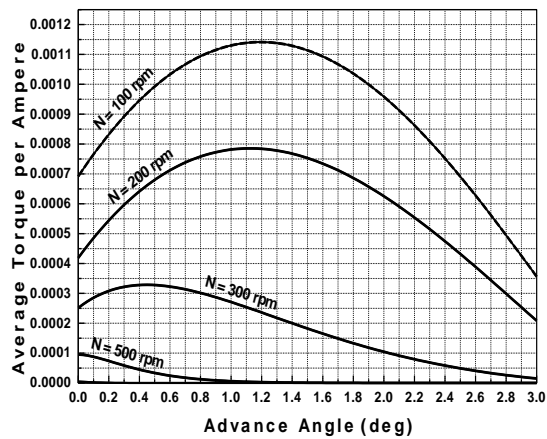
Fig.12 Average torque per ampere versus advance turn-on angle at different speeds
