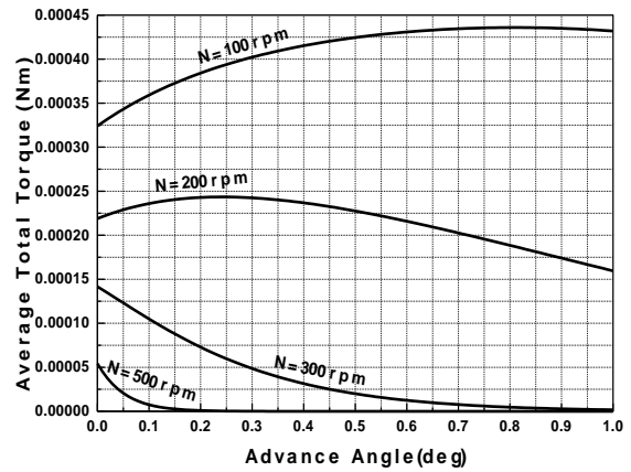
Fig.14 Average total torque versus advance turn-off angle at different speeds
