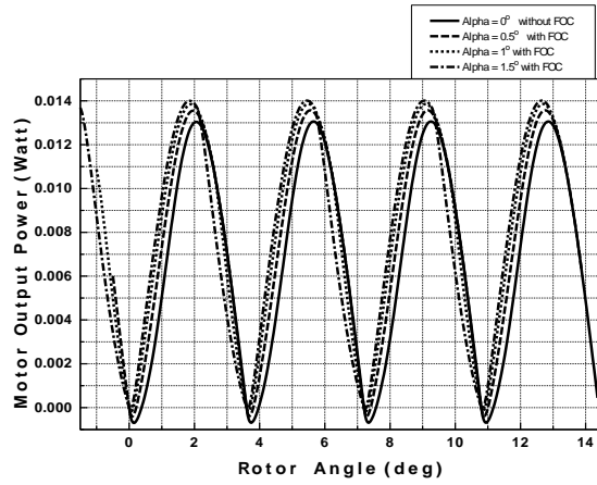
Fig.5 Motor output power versus rotor angle during four step angles
